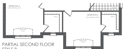
PARTIAL SECOND FLOOR STYLE B
