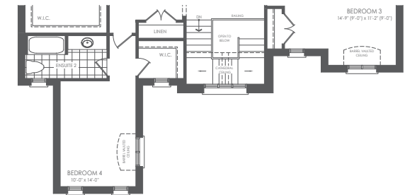
PARTIAL SECOND FLOOR STYLE B
