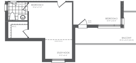
PARTIAL SECOND FLOOR STYLE D
