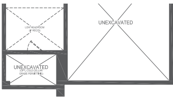
PARTIAL BASEMENT STYLE E
