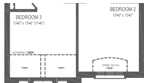
PARTIAL SECOND FLOOR STYLE B
