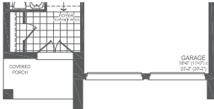
PARTIAL GROUND FLOOR STYLE D
