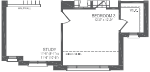
PARTIAL SECOND FLOOR STYLE E
