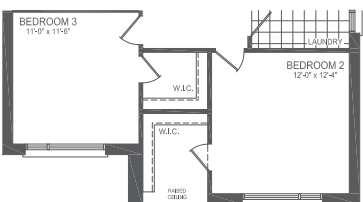
PARTIAL SECOND FLOOR STYLE E
