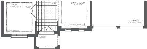
PARTIAL GROUND FLOOR STYLE B
