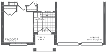
PARTIAL GROUND FLOOR STYLE B FOR LOFT AND NON-LOFT
