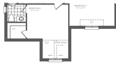
PARTIAL SECOND FLOOR STYLE B
