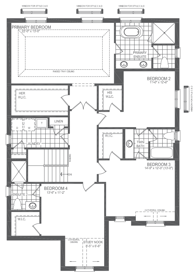
SECOND FLOOR STYLE A
