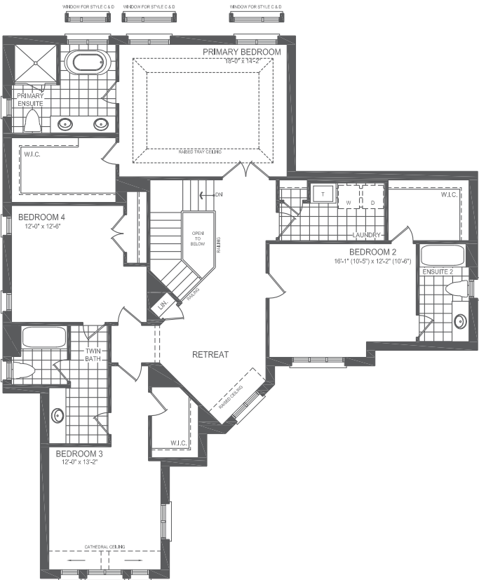
SECOND FLOOR STYLE A
