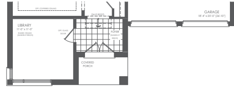
PARTIAL GROUND FLOOR STYLE D
