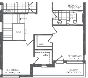
PARTIAL SECOND FLOOR STYLE E
