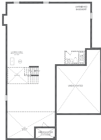
BASEMENT STYLE A / B
