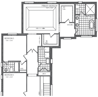
PARTIAL OPT. 5 BEDROOM SECOND FLOOR STYLE D
