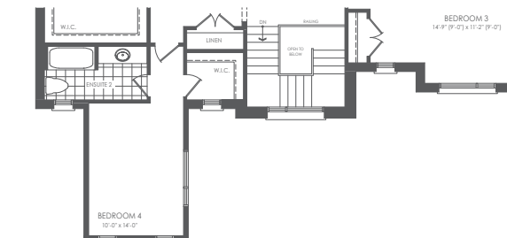
PARTIAL SECOND FLOOR STYLE C
