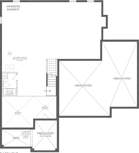
BASEMENT STYLE A
