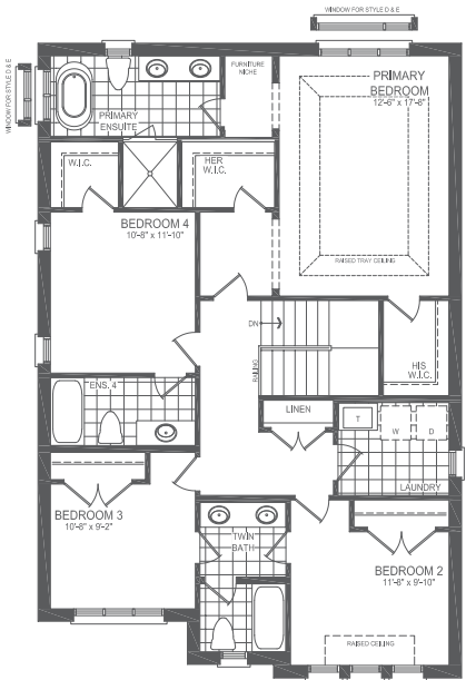
OPT. 3 BATH SECOND FLOOR STYLE B
