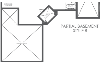
PARTIAL BASEMENT FOR OPT. GROUND FLOOR IN-LAW SUITE STYLE A/B
