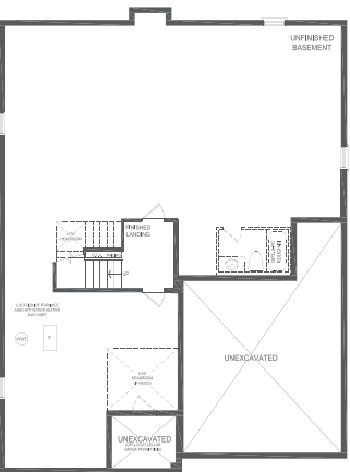
BASEMENT STYLE A FOR NON-LOFT
