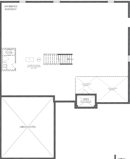
BASEMENT STYLE A FOR LOFT
