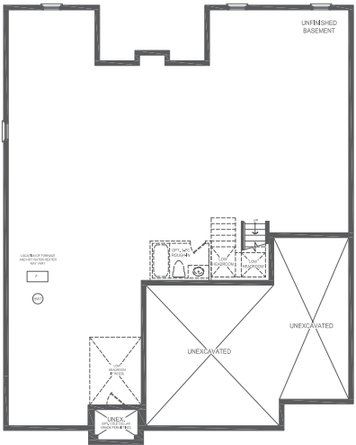
BASEMENT STYLE A/B FOR LOFT
