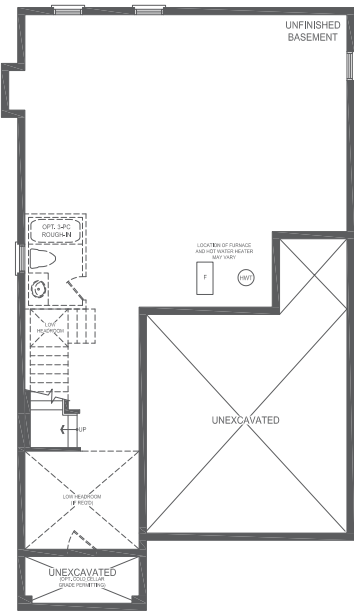
BASEMENT STYLE B, C & D
