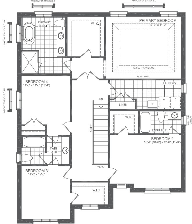
SECOND FLOOR STYLE A
