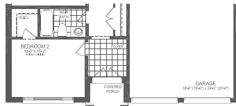
PARTIAL OPT. GROUND FLOOR STYLE D FOR LOFT
