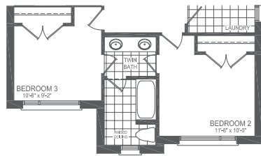
PARTIAL OPT. 3 BATH SECOND FLOOR STYLE E
