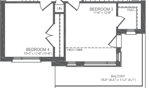
PARTIAL OPT. 5 BEDROOM SECOND FLOOR STYLE D
