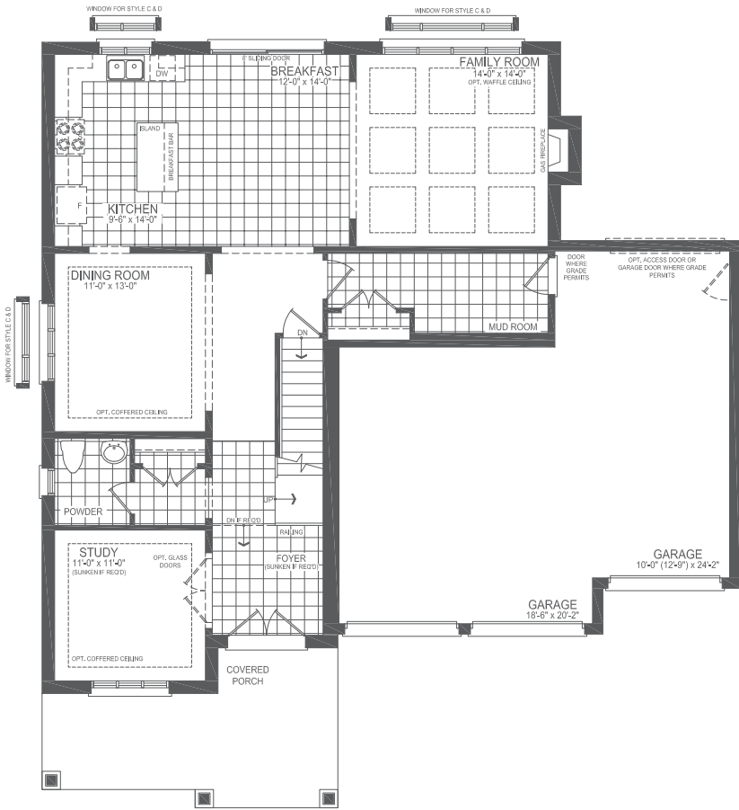
GROUND FLOOR STYLE A
