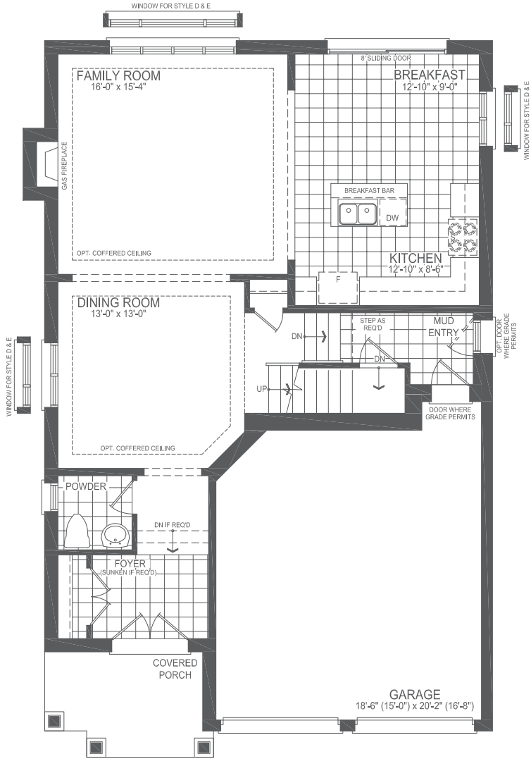
GROUND FLOOR STYLE B & C
